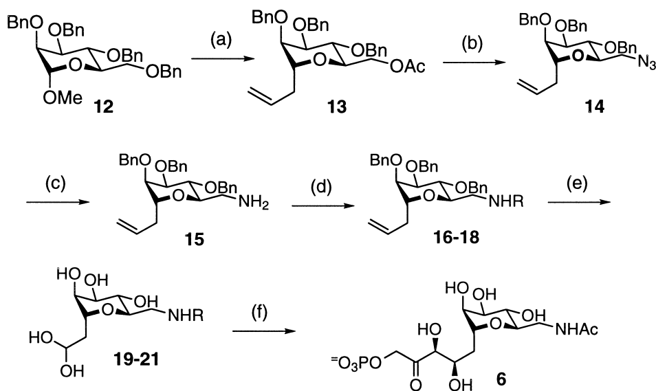
Scheme 1. Conditions: (a) allyl alcohol, cat. CSA, 90 °C, overnight, 80%; (b) (i) \text{O}_3 , \text{CH}_3\text{Cl}/\text{MeOH} = 4/1 , -78^\circ\text{C} ; (ii) \text{PPh}_3 , rt, 72%; (c) pH 6.7, DHAP, RhaA, 31%; (d) pH 6.7, DHAP, FucA, 30%; (e) TsCl, Py, 0 °C, 4 h, 62%; (f) \text{NaN}_3 , DMF, 60 °C, 5 h, 54%; (g) pH 6.7, DHAP, FDPA, 30%.
