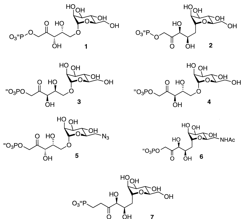
Figure 2. Mannosyl phosphate/phosphonate SLe x mimetics.
