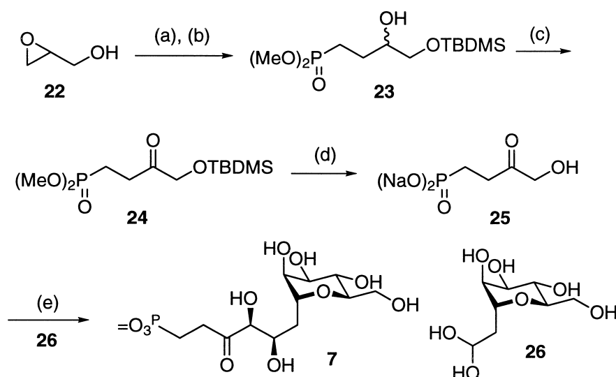
Scheme 3. Conditions: (a) TBDMSCl, imidazol, \text{CH}_2\text{Cl}_2 , 91%; (b) \text{MeP}(\text{O})(\text{OMe})_2 , BuLi, \text{BF}_3 \cdot \text{OEt}_2 , THF, -78^\circ\text{C} , 61%; (c) Dess–Martin reagent, \text{CH}_2\text{Cl}_2 , 68%; (d) (i) TMSBr, \text{CH}_2\text{Cl}_2 ; (ii) NaOH to pH 7.0, 75%; (e) DHAP, RAMA, pH 6.7, 7 days, 25%.
