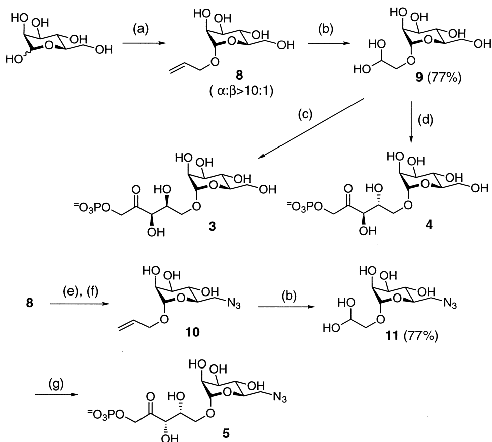
Scheme 1. Conditions: (a) allyl alcohol, cat. CSA, 90 °C, overnight, 80%; (b) (i) \text{O}_3 , \text{CH}_3\text{Cl}/\text{MeOH} = 4/1 , -78^\circ\text{C} ; (ii) \text{PPh}_3 , rt, 72%; (c) pH 6.7, DHAP, RhaA, 31%; (d) pH 6.7, DHAP, FucA, 30%; (e) TsCl, Py, 0 °C, 4 h, 62%; (f) \text{NaN}_3 , DMF, 60 °C, 5 h, 54%; (g) pH 6.7, DHAP, FDPA, 30%.
